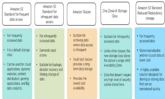
Figure 3: AWS S3 Storage Classes and Their Use Cases (Source: https://www.simplilearn.com )
